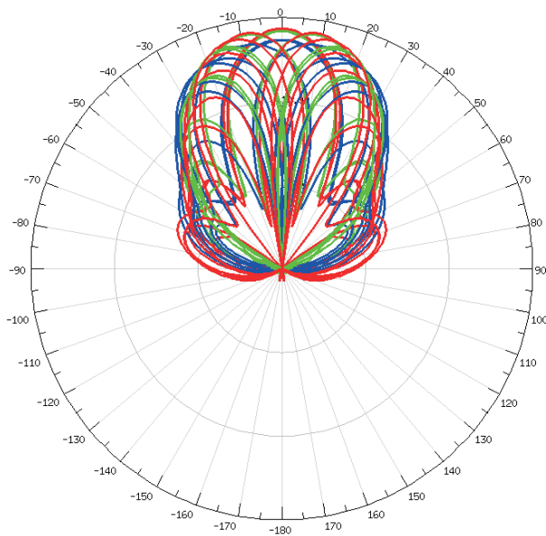
BFM06009 beam array for elevation and azimuth.
