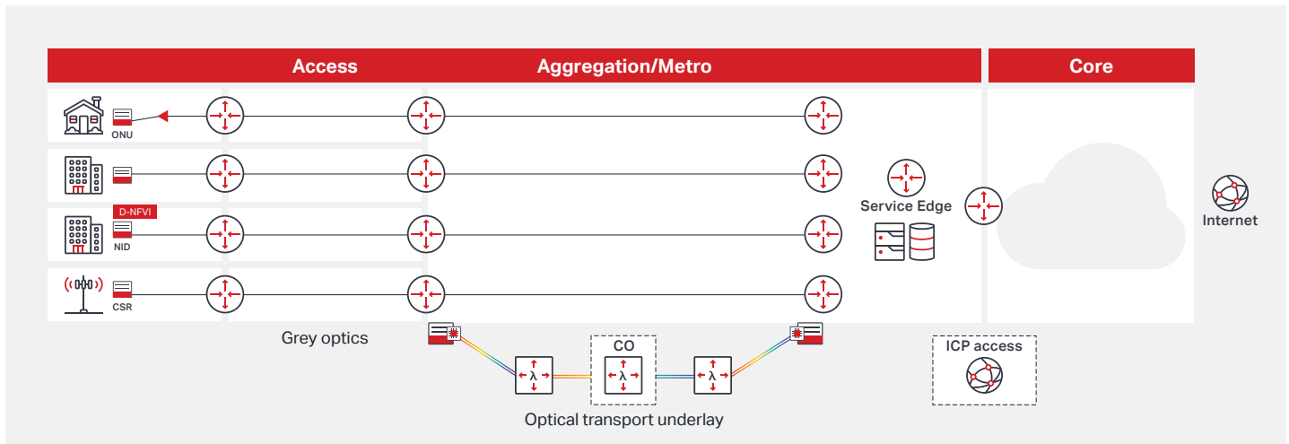
Figure 1. Traditional network design
